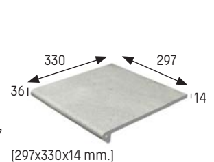
[297x330x14 mm.]
