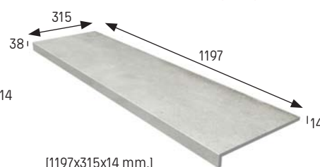
[1197x315x14 mm.]
