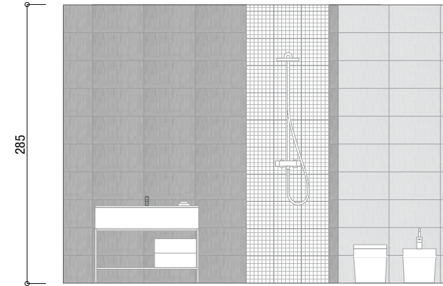
Wall A
