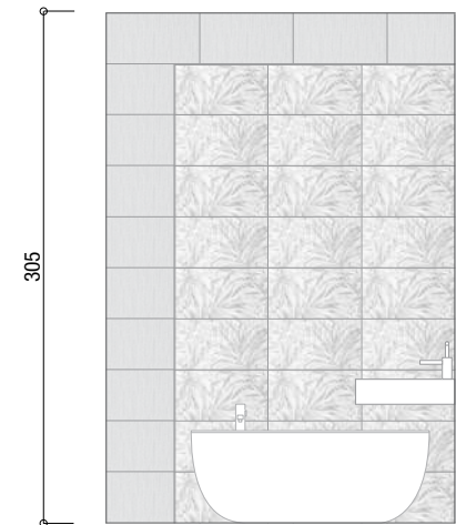
Wall B
