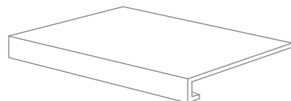
GRADONE - STEP 33x59x3,2x3,2 - 12 15/16 "x23 1/4 "x1 1/4 "x1 1/4 "
